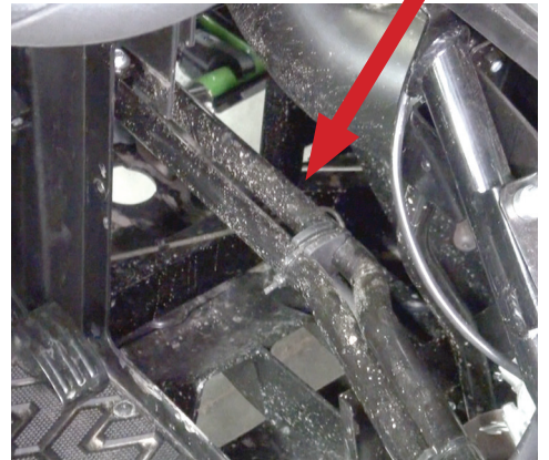
Fig 20 - Wrap these lines. Make sure hook and loop closure is facing away from exhaust
