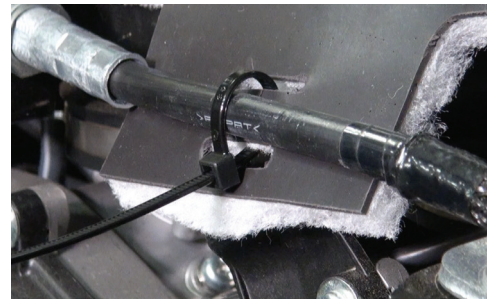
Fig 22 - Secure driver side through slots with zip tie
