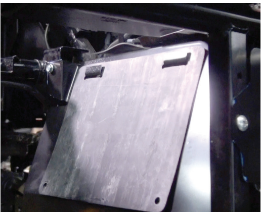
Fig 13 - Remove metal heat shield under drivers seat. The piece with the rubber flap attached to it
