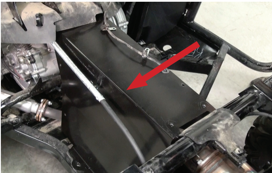
Fig 16 - Remove the driver side and top piece of exhaust tunnel. (one solid piece)
