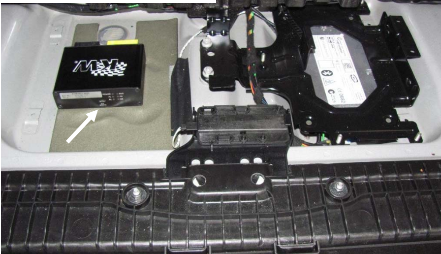
Montageposition 10 / Assembly position 10
