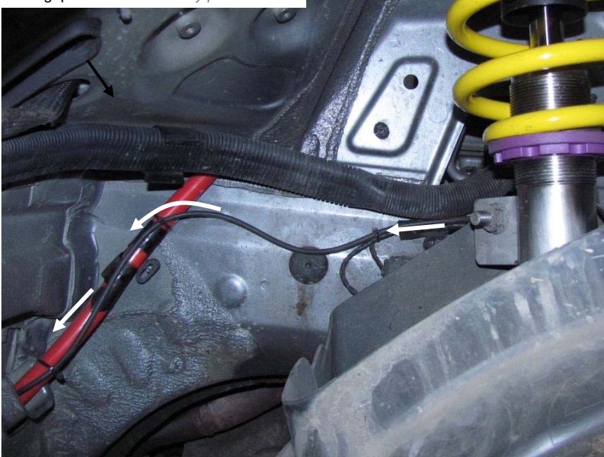
Montageposition 1 / Assembly position 1
