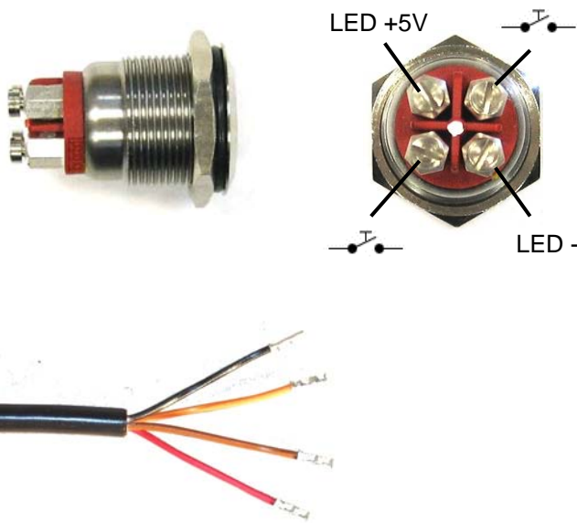
Montageposition 5 / Assembly position 5
