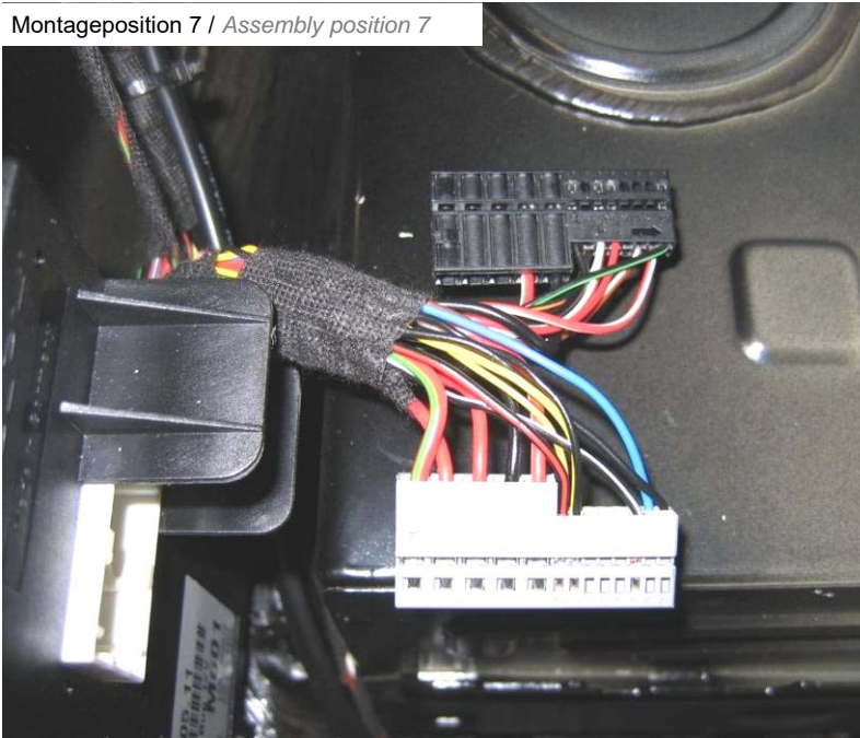
Montageposition 7 / Assembly position 7
