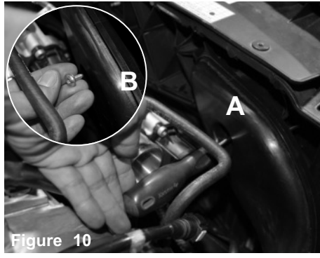
Figure 10 A) Loosen the torx screw on the ram scoop located on the front of the radiator support B) Remove the torx screw from the scoop.
