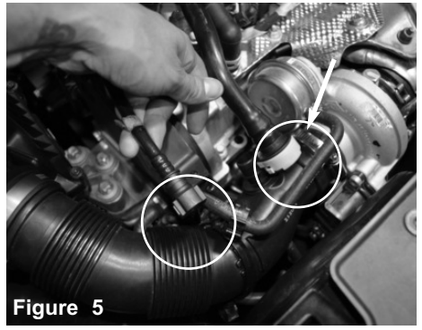
Figure 5 Disconnect both vacuum and crank case line from the factory
