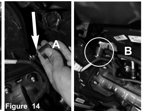
Figure 14 A) Locate the M6 stud in front of vehicle on frame, install the female/male vibramount to the stud. B) Secure and tighten M6 vibra mount.
