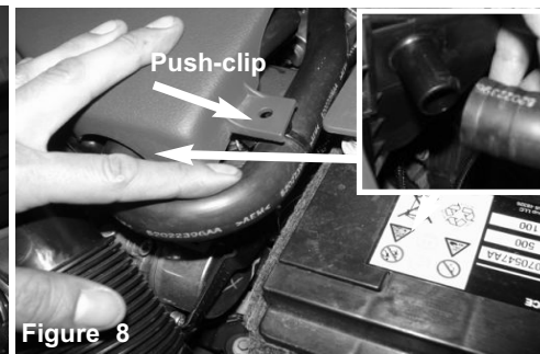
Figure 8 Now push the clip holding in the crank-case line away from the air-box/engine cover. Pull back the crank-case line from the air box.
