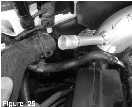
Figure 25 Attach the diverter valve hose to the fitting on the intake tube.
