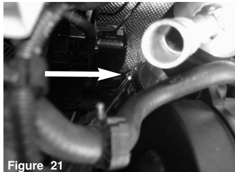
Figure 21 Tighten the remaining clamp on step hose using 8mm nut driver.
