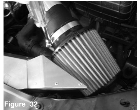
Figure 32 Install the filter and secure using 8mm nut driver.
