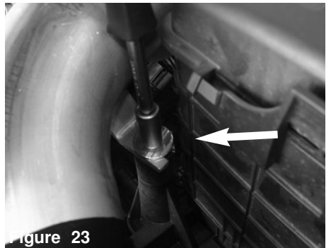
Figure 23 Tighten the nut using 10mm socket and ratchet.
