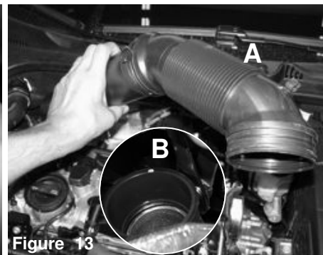
Figure 13 A) Remove intake tube out of vehicle. B) Pinch remaining clamp on turbo and remove.
