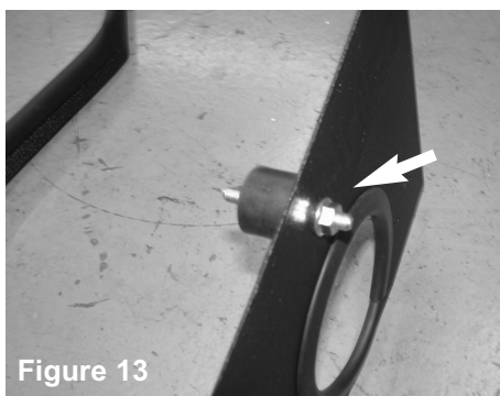
Figure 13 Install the provided vibra mount to the heat shield with vibra mount closes to the engine. Secure using provided m6 nut.
