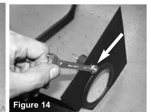
Figure 14 Tighten using 10mm wrench.
