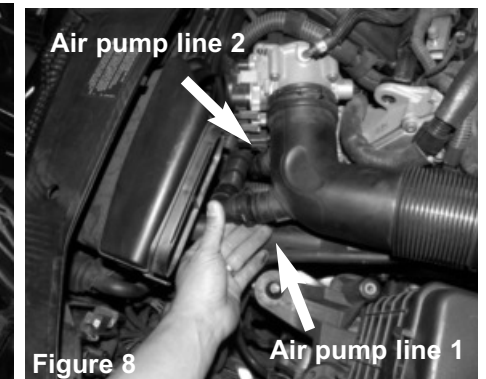
Figure 8 Locate the two air pump lines connect to the throttle body air duct. First disconnect the larger one by firmly pressing on the two release tabs and pulling out and remove the lines.
