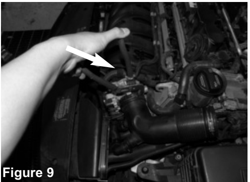
Figure 9 Use a channel lock plier to loosen the pressure clamp on the throttle body and remove the plastic air duct from the throttle body.
