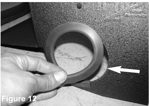
Figure 12 Attach the vinyl trim to the inside of heat shield hole cut out for the intake tube.
