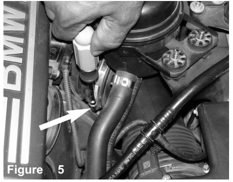
Figure 5 The hose clamp on the air intake duct connected air box cleaner is loosened.
