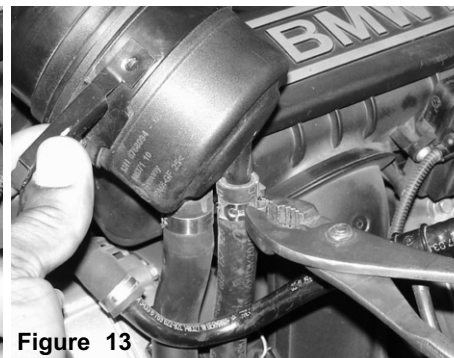
Figure 13 Using a pair of pliers, rotate the clamp quarter turn to the right or counter clockwise. This will prevent any damage to the intake system.
