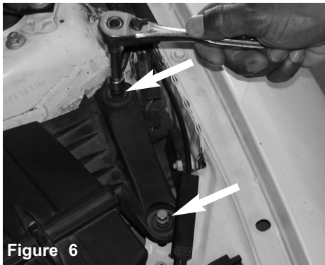
Figure 6 The two 10mm bolts are loosened and removed from the air box bracket.
