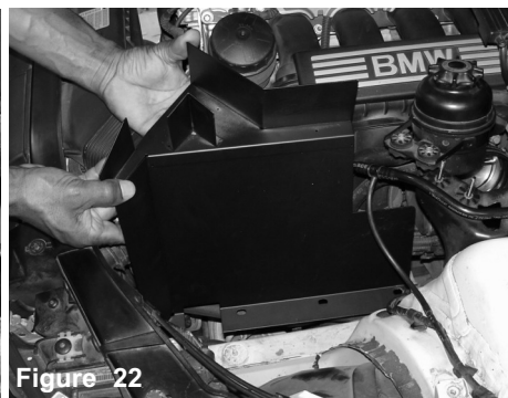
Figure 22 The heat shield is now lowered into the engine compartment.
