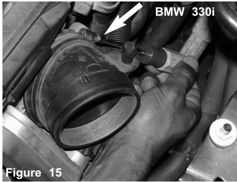
Figure 15 Loosen the throttle body inlet clamp as shown above. The inlet elbow shown above is removed from the 2006 330i
