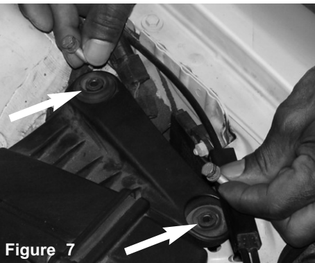
Figure 7 The 10mm bolts are now removed
