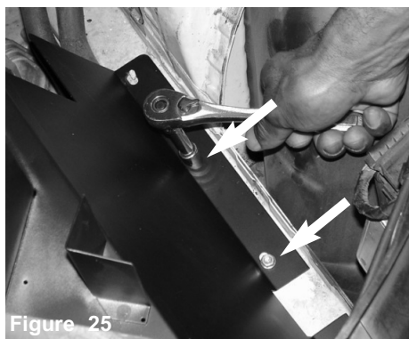
Figure 25 A 10mm socket is used to fasten the flange nuts over the heat shield.
