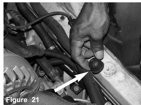
Figure 21 The rubber vibration mount is removed from the car frame as shown above. The new heatshield will be placed over the studs.
