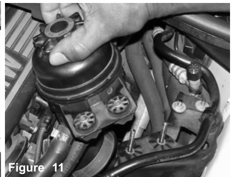
Figure 11 Without disconnecting the two lines, remove the reservoir bottle from the two studs.
