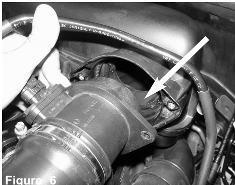
Figure 6 Pull back the MAF sensor housing from the air box.
