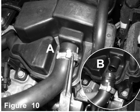
Figure 10 A) With pliers carefully remove the safety clamp on the crank case line. B) Remove the crank case line.
