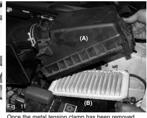
Fig. 11 Once the metal tension clamp has been removed from the throttle body and the two metal clamps have been removed continue to remove the entire air box top (A). Now, remove the top filter panel before moving on to the next step (B).
