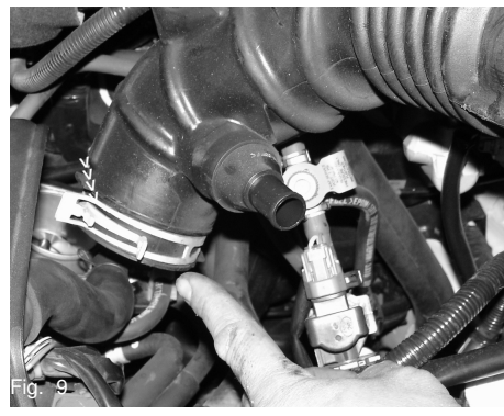
Fig. 9 Use a pair of pliers to depress the metal tension clamp while the air intake duct is pulled off the throttle body as shown above.
