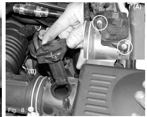
Fig. 8 Unscrew the two screws that secures the mass air flow sensor to the sensor housing (A). Pull the mass air flow sensor up and out of the sensor housing as shown above (B), to be used later in the instruction.
