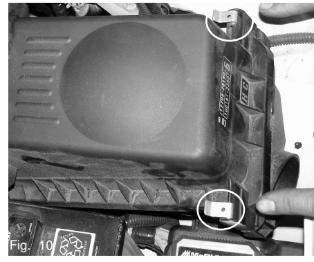
Fig. 10 Pull the two metal clips off the lower box pins and separate the air box top from the air box bottom.
