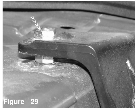
Figure 29 Secure the fuse box by using the stock m6 flange nut as shown above.
