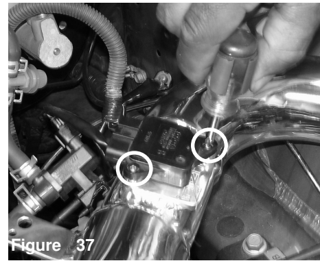
Figure 37 The stock bolts are used to fasten the mass air flow sensor to the machined sensor adapter.
