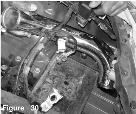
Figure 30 The air intake tube is lowered it into the engine compartment and into the resonator opening, align the intake bracket.
