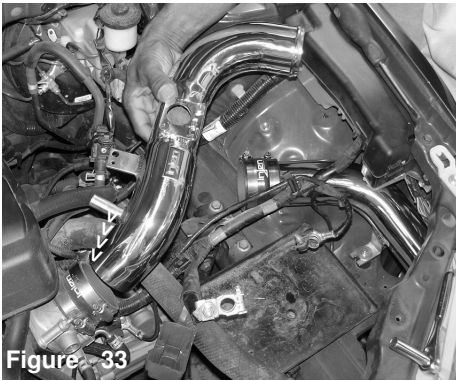
Figure 33 Lower primary intake into the engine comartment. Press the top end of the intake into the throttle body step hose.
