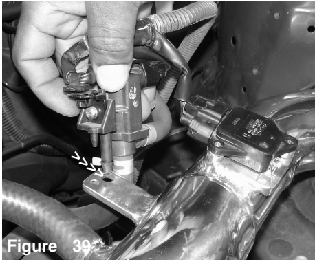
Figure 39 The vacuum switching valve locating pin is now pressed into the flat intake bracket.
