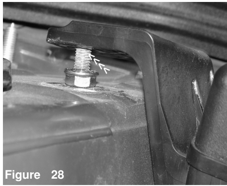
Figure 28 Place the fuse box lip over the stud. The entire fuse box is now raised making room for the air intake.
