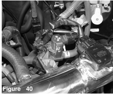
Figure 40 The vacuum switching valve is now sitting flush on the flat bracket.
