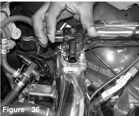
Figure 36 Take the mass air flow sensor and insert it into the machined sensor adapter. Use a dab of light oil on the O-ring, this will insure a good seal.
