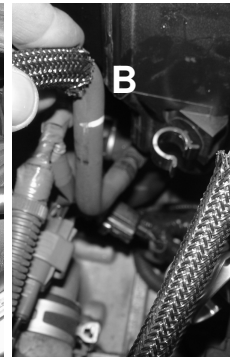
Figure 20 A) Loosen the clamp on the throttle body using 10mm socket or ratchet. B) Pull back any lines from the stock intake system that are attached.
