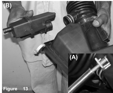
Figure 13 Loosen the clamp on the air intake duct that connects the crankcase vent box (A) from the air intake duct as shown above (B).
