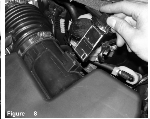
Figure 8 Once you have removed the two bolts, continue to pull the mass air flow sensor out of the sensor housing. This mass air flow sensor will be used later in the installation.
