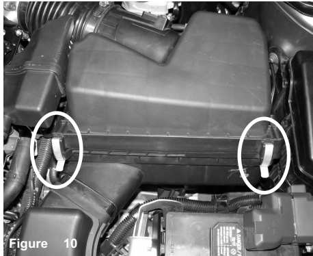
Figure 10 These are the two metal clips that are to be removed from the air box. These two clips connects the top air box to the lower air box.
