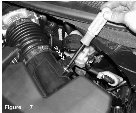
Figure 7 Unscrew the two bolts that secures the mass air flow sensor to the sensor housing.
