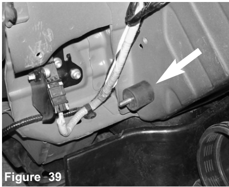
Figure 39 Vibra mount screwed in place.
