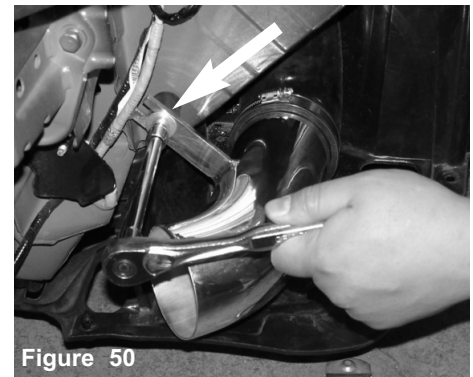
Figure 50 Use a 10mm 3/8 socket and ratchet to tighten the M6 nut.
