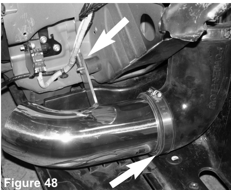
Figure 48 The secondary intake bracket is attached to the vibra-mount stud. The intake is firmly placed into the 3 1/2" 90 degree elbow.
