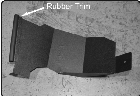
8. Attach the rubber trim to the top of the heat shield. See last steps 25/26 for CVT transmission install.
