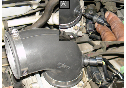
Take air temperature sensor and press it into the grommet located in the 90 degree elbow(A). The air temperature sensor is now installed.
