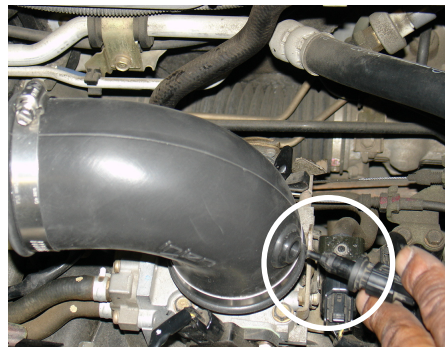
Take the air temperature sensor and press it into the grommet placed in the 90 degree elbow.
