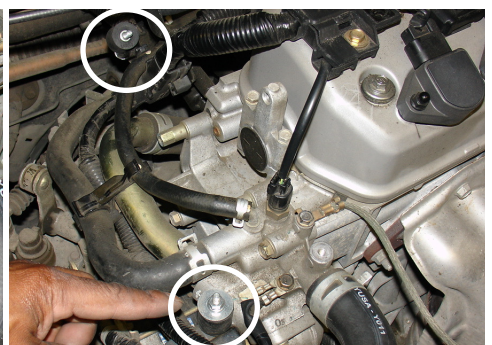
Both vibra-mounts are now installed and ready for the next step.
