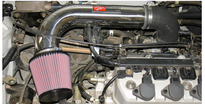
The filter is pressed over the end of the primary intake and used as a short ram. Injen recommends using the short ram in rainy days in order to avoid hydrolocking.
