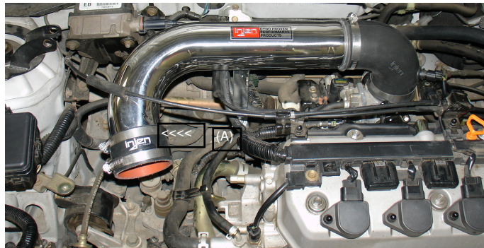
To continue the installation of the cold air intake take the 3" straight hose and press it over the end of the primary intake. Use two clamps on the hose but only tighten the clamp on the intake side (A).
