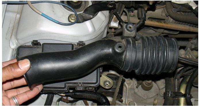
Remove the stock air intake duct connected from the box to the throttle body.
