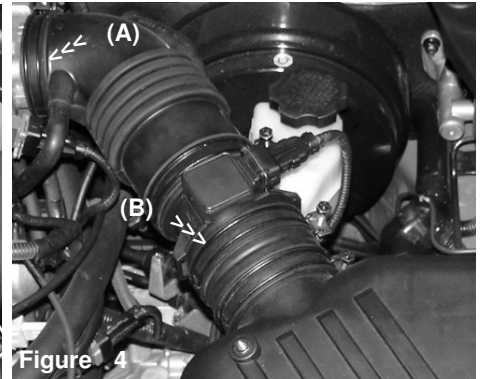
Figure 4 Loosen clamps that secures the air intake duct to the throttle body (A) and the air box cleaner to the lower air intake duct (B).
