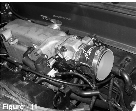
Figure 11 Press the step hose over the throttle body and use two power bands on the hose, tighten the band on the throttle body side for now.
