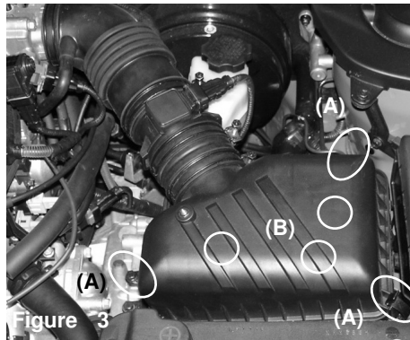
Figure 3 Remove top clips from lower air box (A) Once clips have been removed, lift the top cover and remove the inside panel filter. Loosen and remove the three bolts on the lower air box fastened to the motor mount (B).
