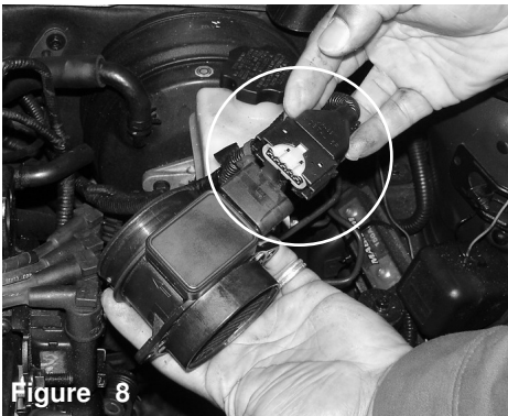
Figure 8 Depress end clips on the electrical harness clip and pull the clip away from the mass air flow sensor.
