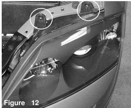
Figure 12 Remove the two bolts from the tabs on the head lamp. Once bolts have been removed, continue to pull the head lamp out of the frame.
