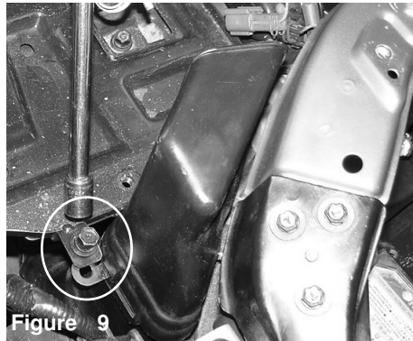
Figure 9 Remove the m6 bolt located on the corner battery tray. Once you have removed the bolt, gently pry the top resonator box loose.
