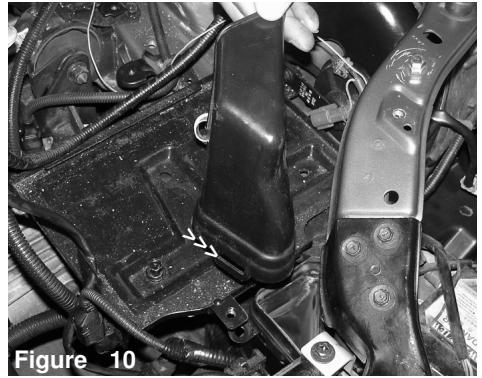
Figure 10 The tabs with the holes are used to hook into the notch located in the resonator box as shown above.
