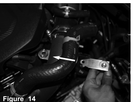
Figure 14 Lift the factory upper intercooler pipe up and slide the stainless bracket underneath the upper intercooler pipe bracket. Re-install the bolt from step 12.
