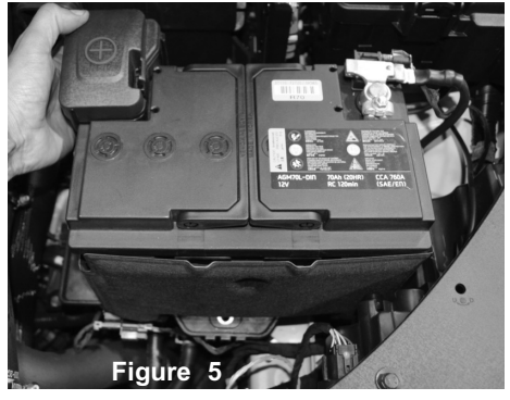
Figure 5 Loosen the battery bracket and pull battery forward. This will allow removal the the OEM air box.
