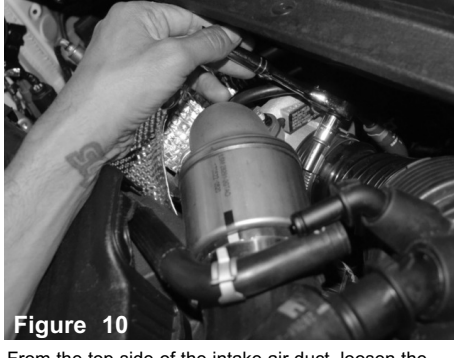
Figure 10 From the top side of the intake air duct, loosen the clamp with a 10mm socket/ratchet attached to the turbo inlet. Detach the intake air duct from the turbocharger and you may now remove the intake air duct from the engine bay.
