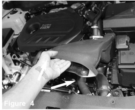
Figure 4 Use a 10mm socket/ratchet and remove the two M6 bolts attached to the factory air box inlet duct. Remove the air box inlet duct from the engine bay. This air duct will be re-used in this installation to draw in cool air to the Injen intake system.
