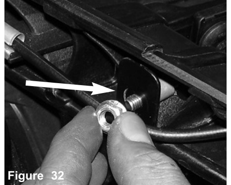
Figure 32 The m6 flange nut is used to tighten the reservoir bracket in place. Note: The 3/16" spacer between the bracket and cross member, used to support the bracket to keep it from distorting.
