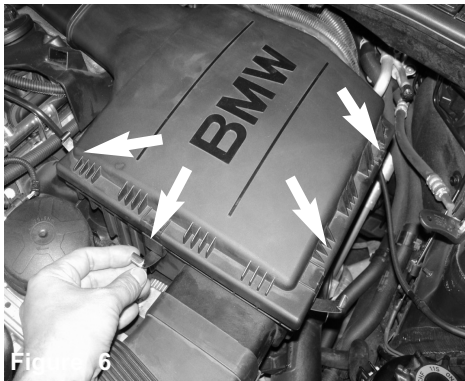
Figure 6 Un-clip the 4 tabs holding in the upper half of airbox.
