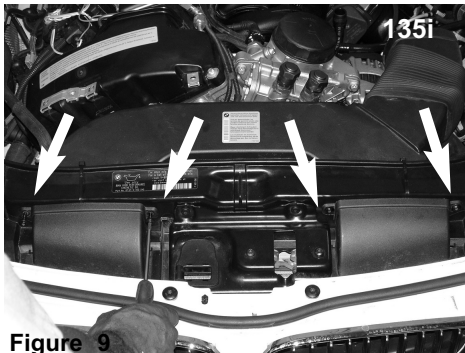
Figure 9 For the 135i only loosen and remove the four bolts holding the primary air scoops in place using t25 torx bit.
