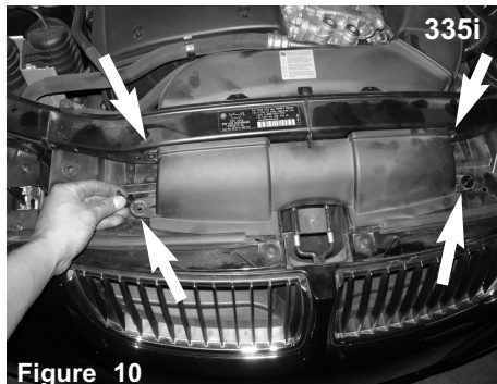
Figure 10 For the 335i loosen and remove the 2 bolts and 2 plastic push clips holding in the primary 1 piece air scoop using t25 torx bit.
