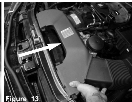
Figure 13 Lift up and pull back the the lower primary air scoop assembly.
