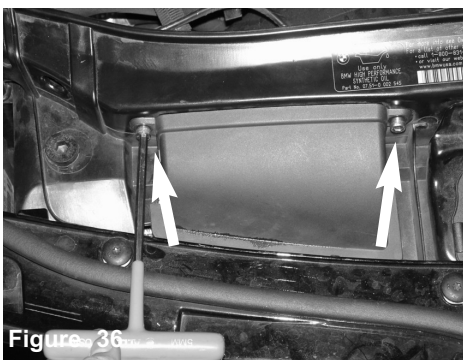
Figure 36 Secure the passenger factory side scoop using the M6 button head screws and 2 flange nuts behind the core support.
