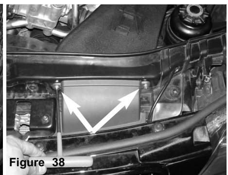
Figure 38 Tighten the 2 screws using allen key and secure. Note: This does not require the use of the air scoop bracket only, for the 335i.
