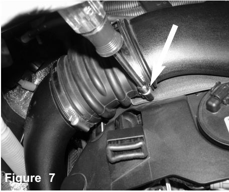
Figure 7 Loosen the clamp on intake tube using 7mm nut driver.
