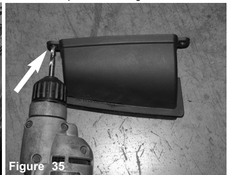
Figure 35 Drill all the 4 holes out to 1/4" on the factory scoops to make the M6 screws able to pass through.
