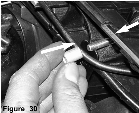
Figure 30 The 3/16" aluminum spacer is slipped over the m6 x 35mm bolt used to secure the reservoir bracket.
