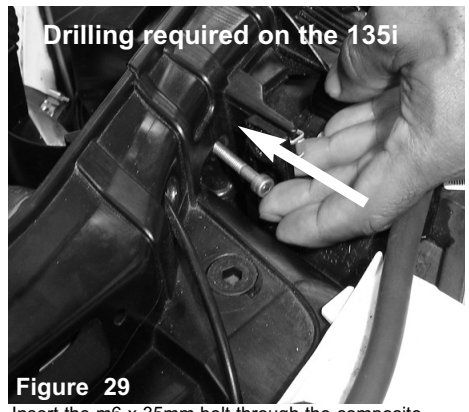
Figure 29 Insert the m6 x 35mm bolt through the composite cross member and through the 3/8" aluminum coupler as shown in figure 26.
