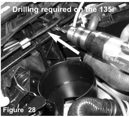
Figure 28 Applicable to the 135i only: Use a 1/4" drill bit to drill a hole through the composite cross member, the short bracket on the cup is used as a pattern.
