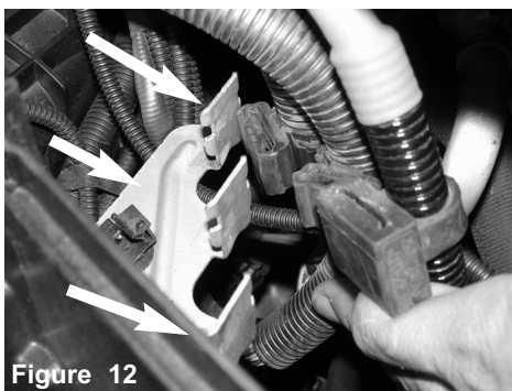
Figure 12 Pull back the 3 harness lines attached to the lower air box assembly.
