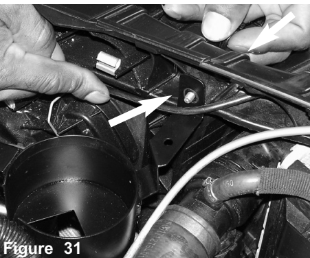
Figure 31 The m6 x 35mm hex bolt is inserted through the cross member, and into the 3/8" aluminum coupler. The aluminum coupler is used as a back support for the reservoir bracket as shown in figure 28.
