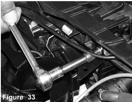
Figure 33 A 10mm socket and ratchet is used to fasten the flange nut to the m6 bolt.
