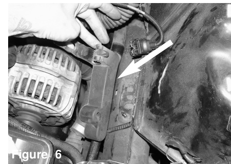
Figure 6 Remove the rubber isolator from the vehicle frame near the alternator
