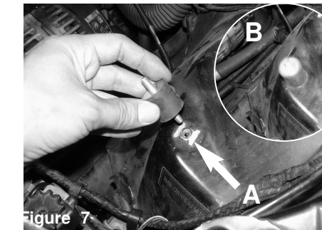
Figure 7 A) install m6 vibramount to the threaded insert on frame from step 5. B) Secure and tighten the vibramount.
