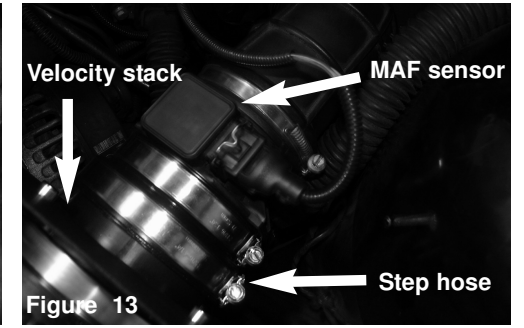
Figure 13 Place the 3.50"-3.75" step hose, #56 and #64 clamp and place the 3.75" hose end on the velocity stack. Now place the MAF sensor into the 3.50" hose end and then secure all clamps
