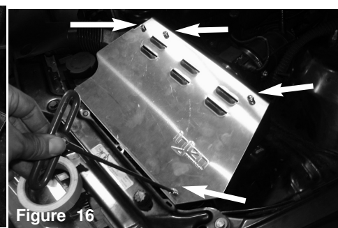
Figure 16 Place the four M6 allen screws onto the heatshield cover and secure the cover to the heatshield with a allen driver. *Unfinished cover shown for illustrative purposes only. Wrinkle black finish will be standard.
