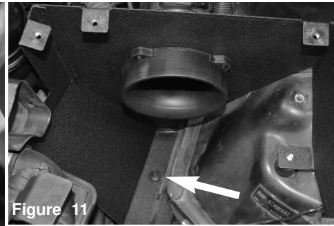
Figure 11 Place the heatshield into the engine bay. Place the grommet onto the threaded stud located on the frame rail near the shock tower
