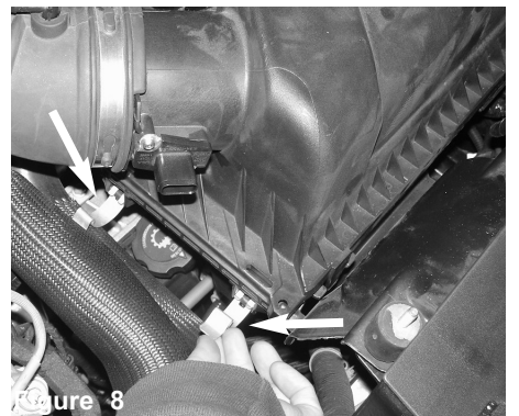
Unlatch the two retaining clips located on the left side of the air box assembly.
