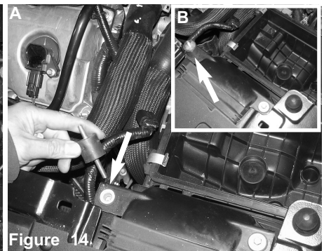
Figure A: Use a Torx driver to remove the two screws from the MAF sensor located on the upper air box assembly. Figure B: Remove the MAF sensor from the upper air box housing.
