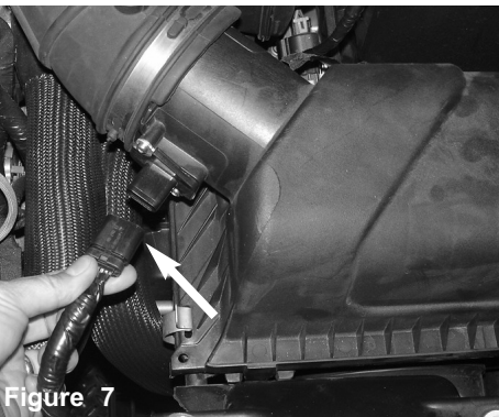
Disconnect the MAF sensor harness from the MAF sensor located on the top factory air box assembly.
