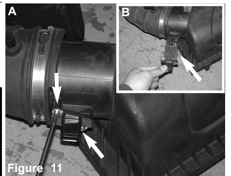
Figure A: Use a Torx driver to remove the two screws from the MAF sensor located on the upper air box assembly. Figure B: Remove the MAF sensor from the upper air box housing.
