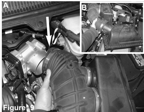
Figure A: Detach the air duct from the throttle body. Figure B: Now remove the entire upper portion of the air box assembly
