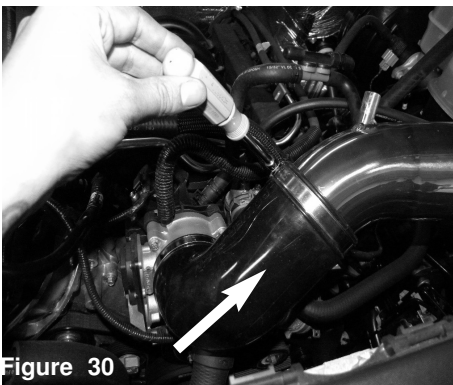
Figure 30 Position for the best possible fit. Now tighten the clamps on elbow hose using 8mm nut driver.
