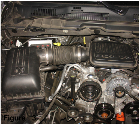
Figure 3 Stock engine compartment
