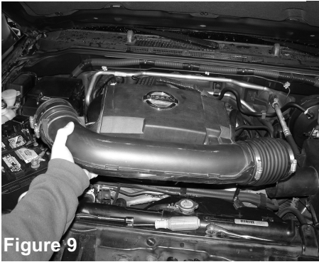
Figure 9 With both clamps loosened, remove entire air duct with the air resonator box attached.
