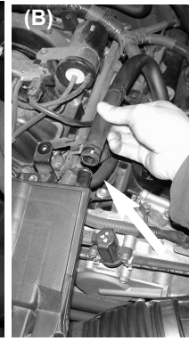
Figure 7 (A) Loosen tension clamp with a plier. (B) Then remove vacuum breather line from air duct resonator box.
