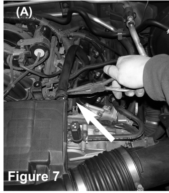
Figure 7 (A) Loosen tension clamp with a plier. (B) Then remove vacuum breather line from air duct resonator box.
