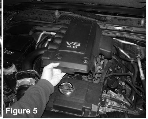
Figure 5 Lift up and pull towards you to remove the engine cover. This cover is removed to access the two 10mm bolts to the air duct resonator box/
