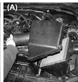
Figure 10 (A) Unclip air mass sensor harness (B) Then use a phillips screw driver to remove the two screws holding the MAF sensor to the housing. These screws will be re-used.
