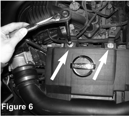
Figure 6 Loosen and remove the two 10mm bolt located on the air duct resonator box.
