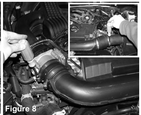
Figure 8 Use a 8mm nut driver to loosen clamp on throttle-body side air duct and air box side
