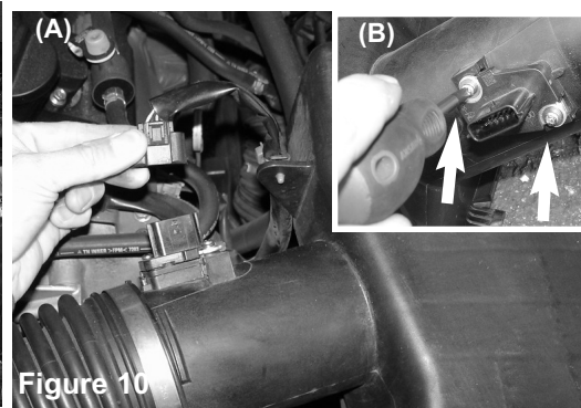
Figure 10 (A) Unclip air mass sensor harness (B) Then use a phillips screw driver to remove the two screws holding the MAF sensor to the housing. These screws will be re-used.
