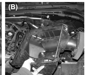
Figure 11 Now remove the MAF sensor out of the factory air box sensor housing. This MAF sensor will be reused later.
