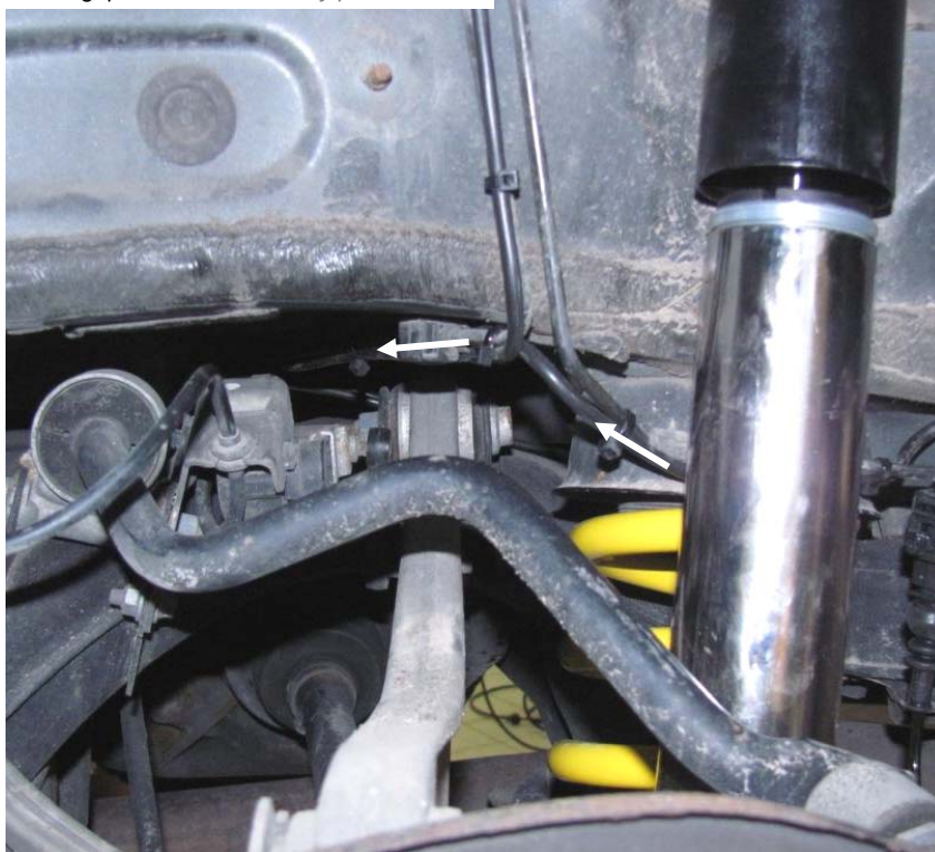
Montageposition 4 / Assembly position 4
