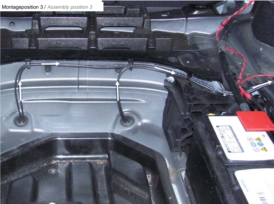
Montageposition 3 / Assembly position 3
