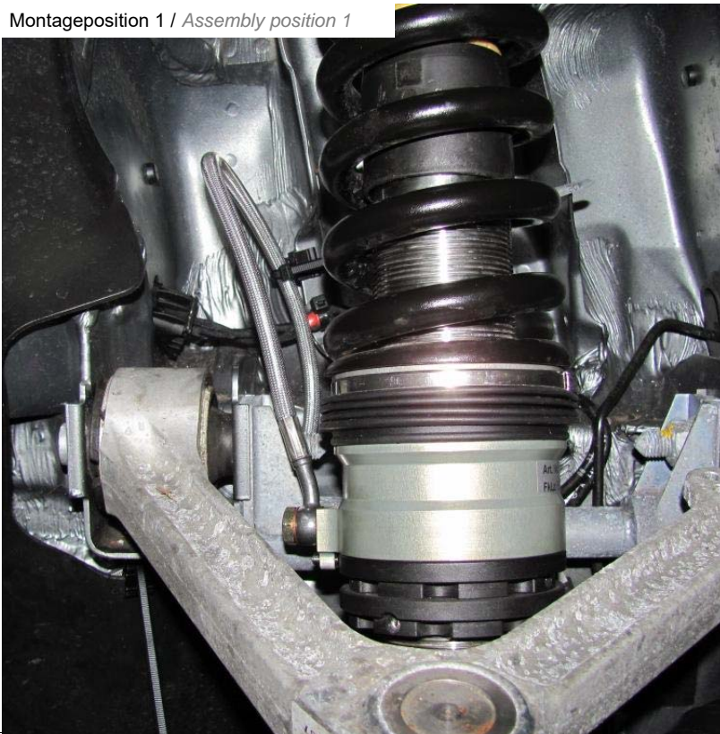
Montageposition 1 / Assembly position 1
