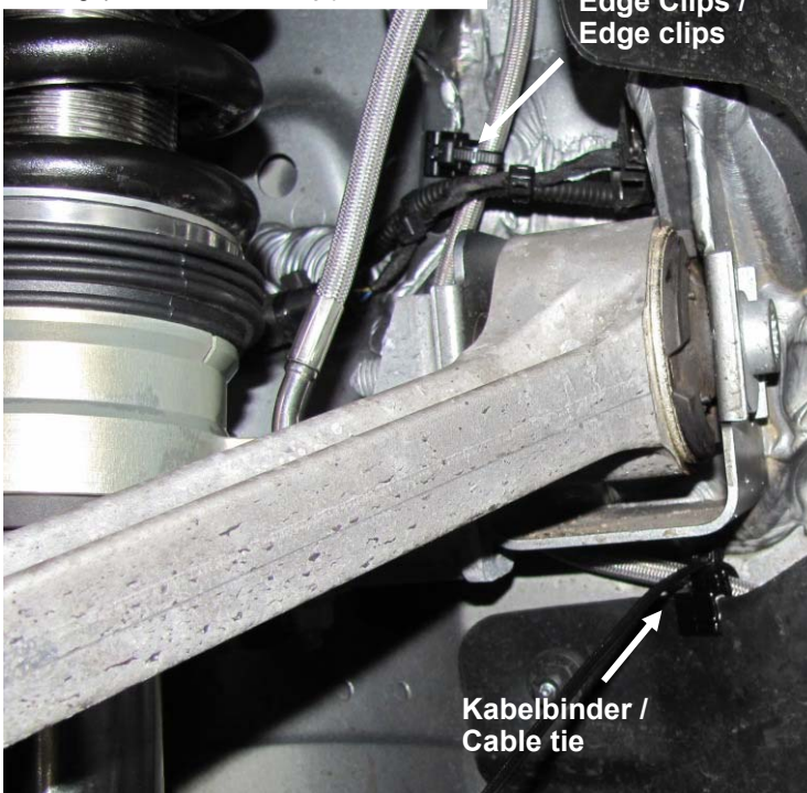
Montageposition 2 / Assembly position 2
