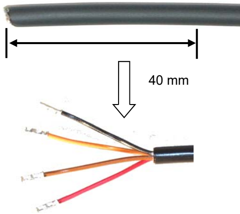
Montageposition 9 / Assembly position 9
