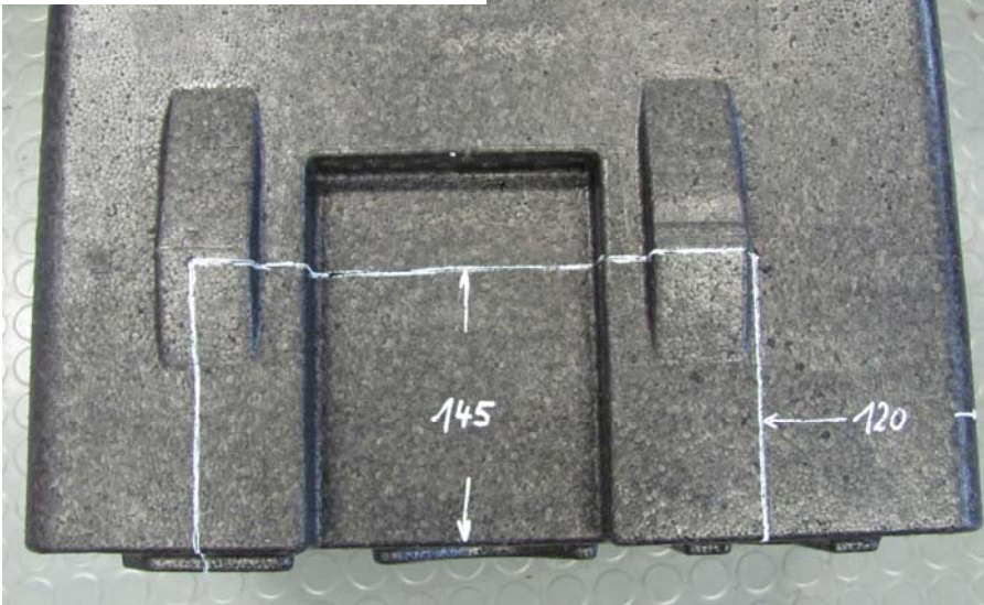
Montageposition 3 / Assembly position 3
