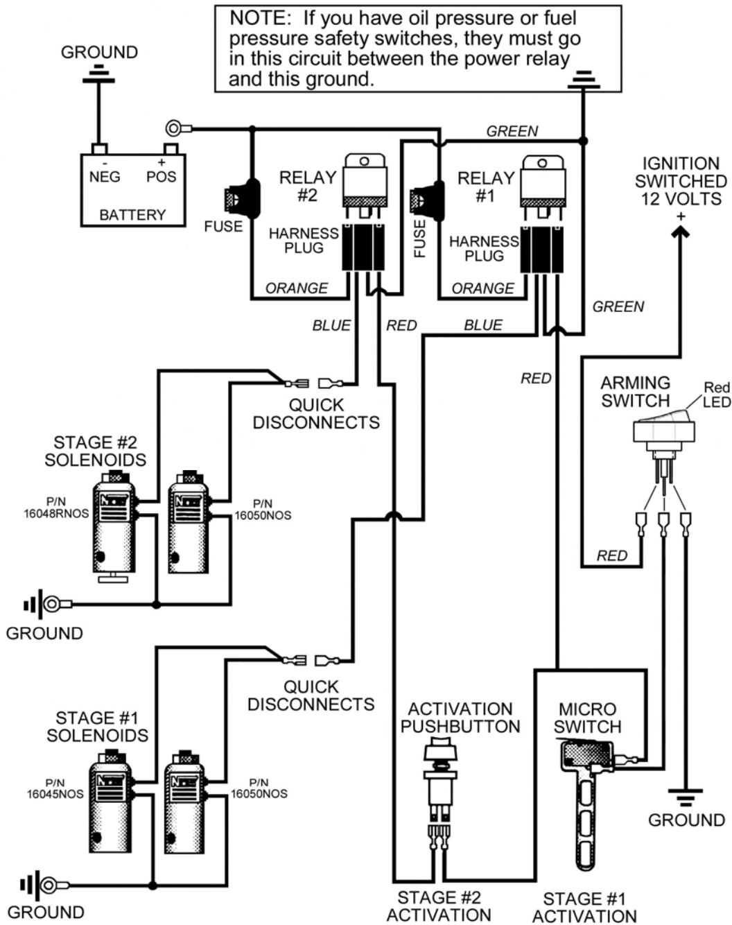
Figure 7 Wiring Schematic
