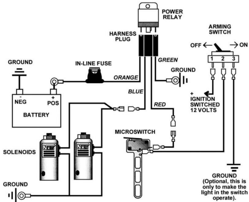
Figure 3 – Microswitch Wiring
