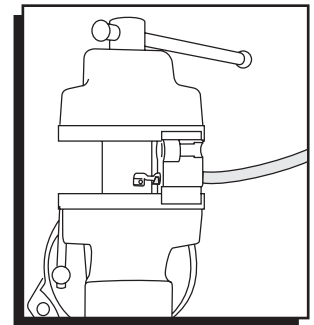
Figure 8 Crimping with the Vise.
