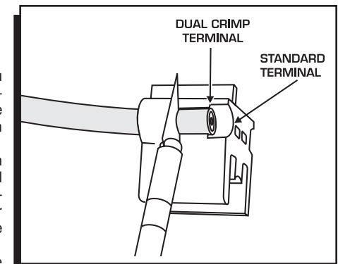
Figure 2 Stripping the Sleeve.
