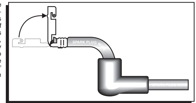
Figure 9 Installing the Boots.
